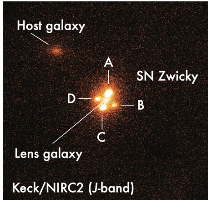
Figure 1. Quadruply-lensed SN Zwicky
