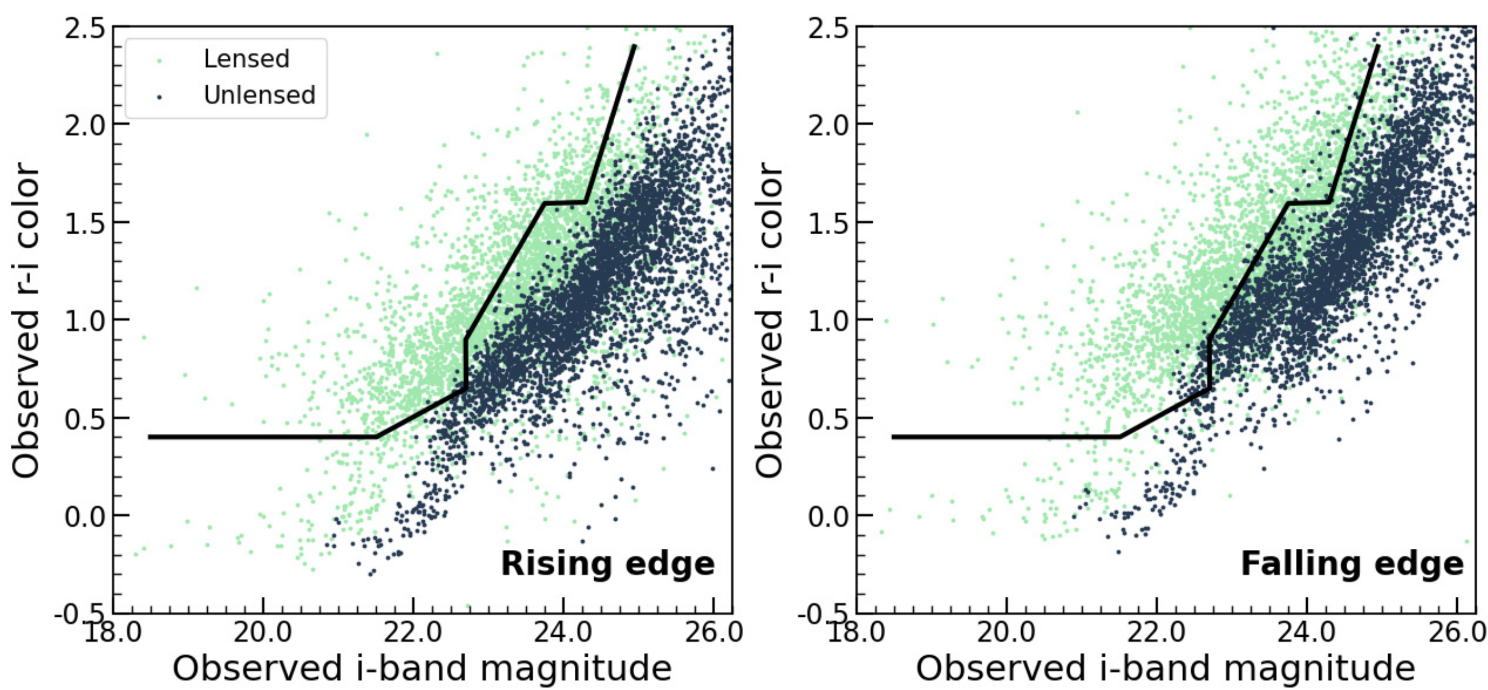
Figure 2. CMD for simulated unlensed (dark blue) and lensed (green) SNIa. We compare the photometric data recorded on rising (left pane) and falling (right panel) phase of the SNIa. The proposed bold black curve, the "red" limit, allows demarcation of the CM space between the lensed and the unlensed SNIa for SNIa both in the rising and falling phase.
