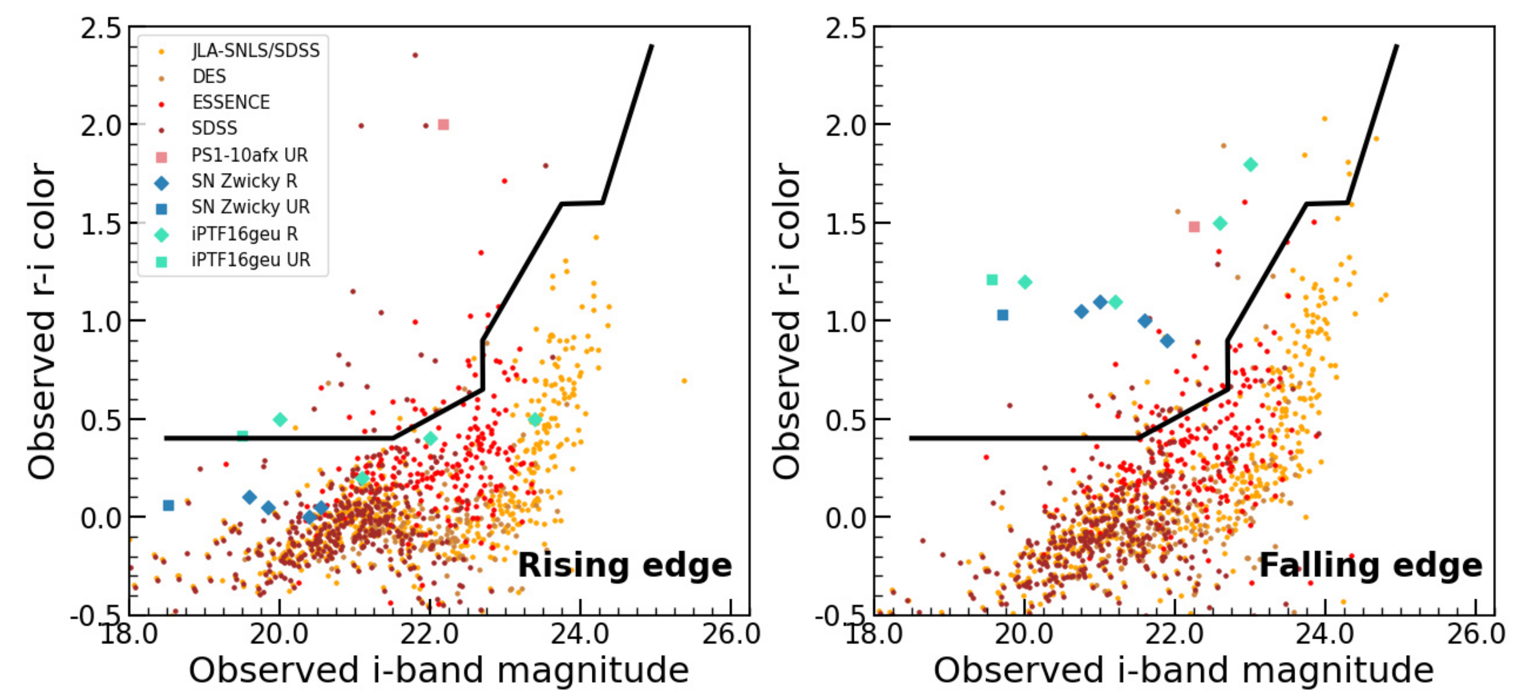
Figure 3. CMD for observed unlensed and lensed SNIa. Photometric data of the observed unlensed SNIa (circles), observed resolved lensed SNIa (diamonds), and unresolved lensed SNIa (squares) in the CMD are shown. The proposed bold black curve (same as in Figure 2) roughly succeeds in eliminating unlensed SNIa during both the rising and falling phases and selects lensed SNIa, as outliers, mainly in the falling phase.
