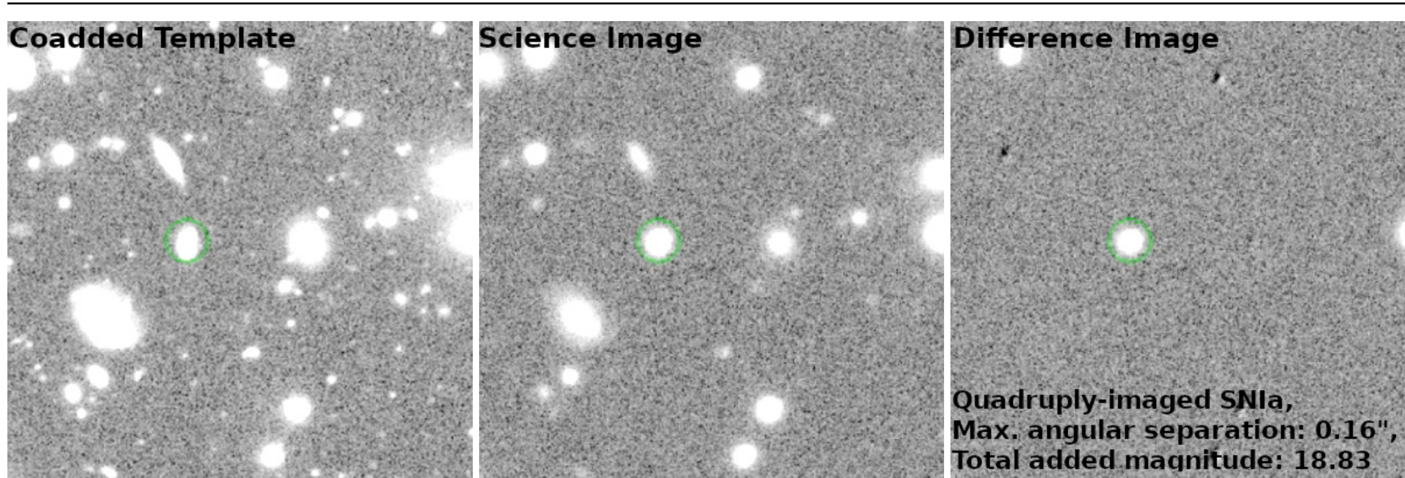
Figure 4. Detection results of our pipeline for an injected lensed SNIa event. The coadded template (left) prior to the SNIa going off shows the foreground lensing galaxy, science exposure (middle) shows the injected quadruply lensed SNIa where the multiple images are unresolved. Difference image (right) shows successfully recovered lensed SNIa (green circle radius of 2") by the DI pipeline.
